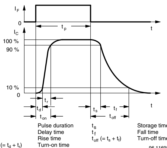
Fig. 4 - Switching Times
