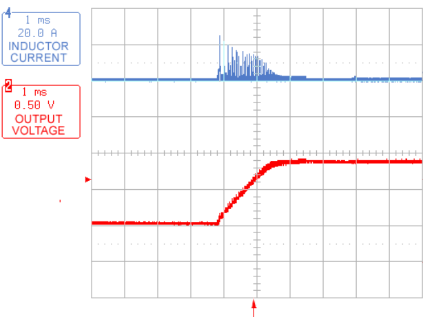
FIGURE 7. PRE-BIASED START-UP IN DCM MODE
