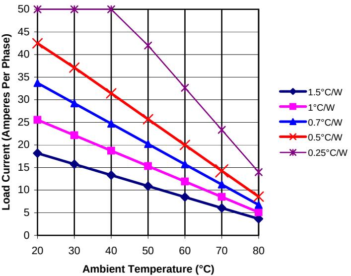
DERATING CURVES: GN0 - 50AMPS
