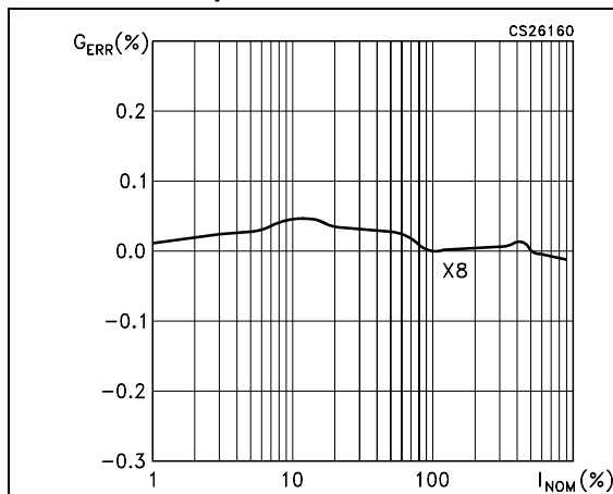
Figure 13. Gain response of \Delta\Sigma AD converters
