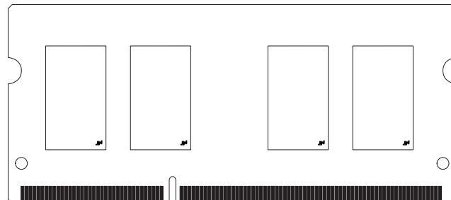
Figure 1: 204-Pin SODIMM (MO-268 R/C C)
