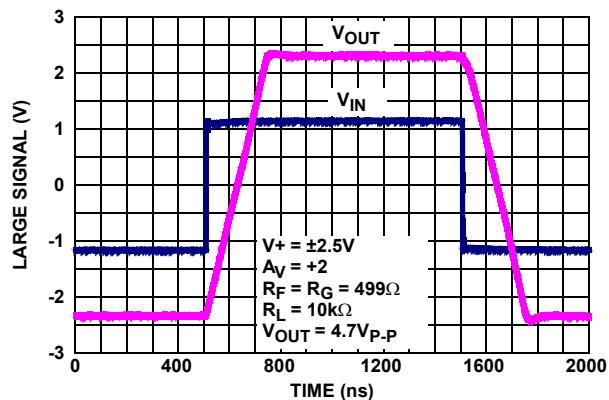
FIGURE 19. LARGE SIGNAL (4.7V) STEP RESPONSE
