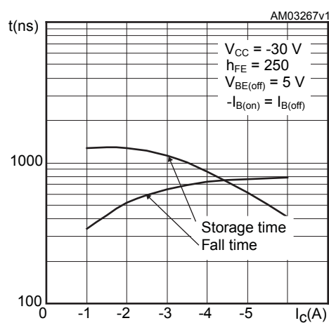
Figure 14. Resistive load switching time (PNP, off)
