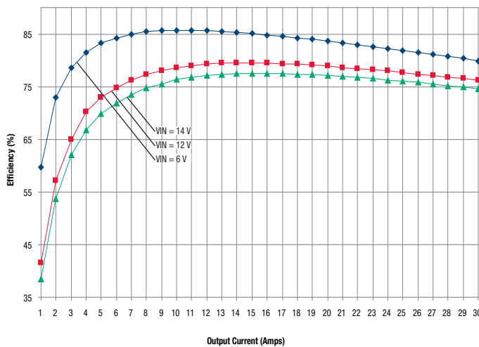
Efficiency vs. Line Voltage and Load Current @ 25°C (V OUT = 0.8V)
