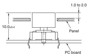
Reference Dimensions
