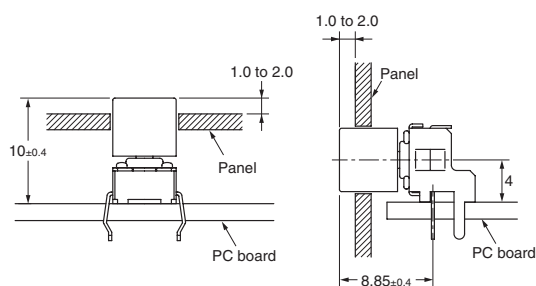
Reference Dimensions
