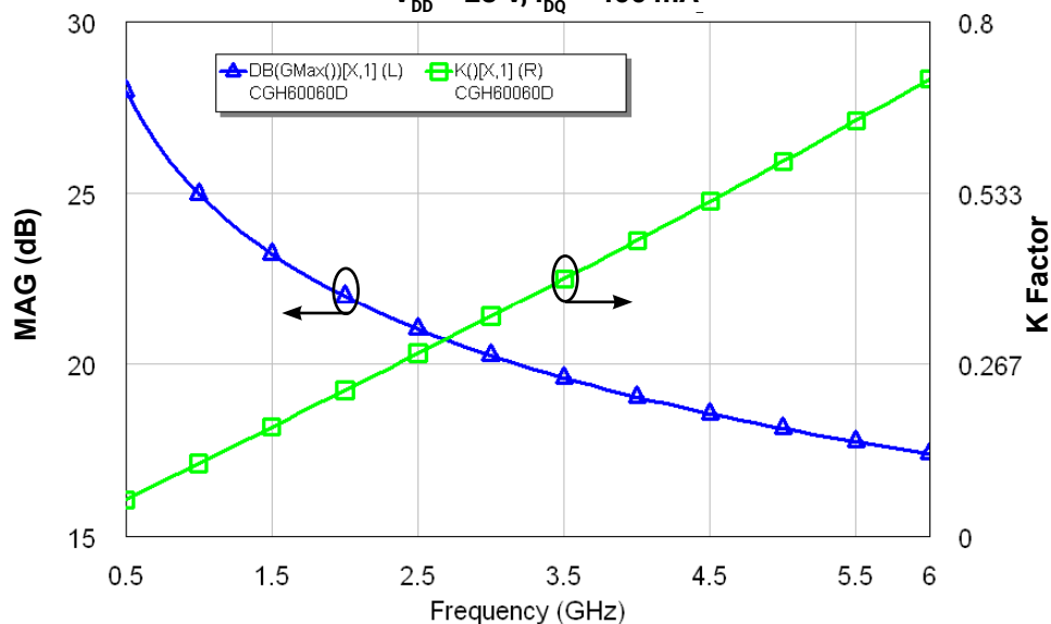
Simulated Maximum Available Gain and K Factor of the CGH60060D
