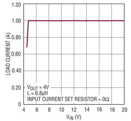
Maximum Buck Load Current
