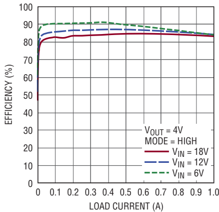
Buck Efficiency
