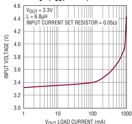
Typical Minimum Buck Input Voltage ( V_{OUT} = 3.3V )
