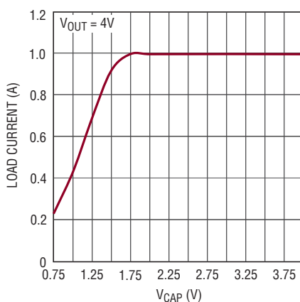
Maximum Boost Load Current
