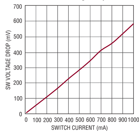
Buck Switch Voltage Drop
