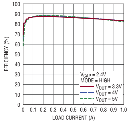
Boost Efficiency
