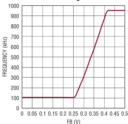
Buck Frequency vs Feedback Voltage
