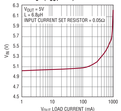
Typical Minimum Buck Input Voltage ( V_{OUT} = 5V )
