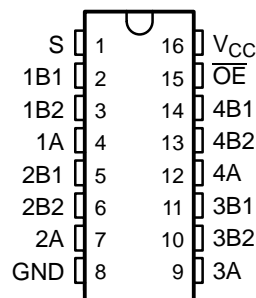
DGVR OR PW PACKAGE (TOP VIEW)
