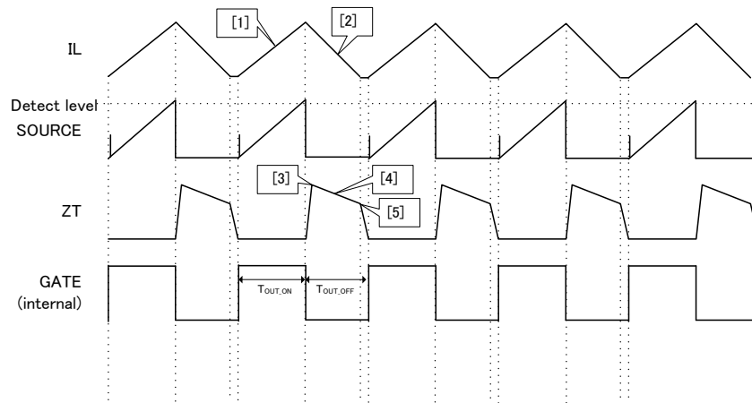
Figure 7. Dimming Waveform
