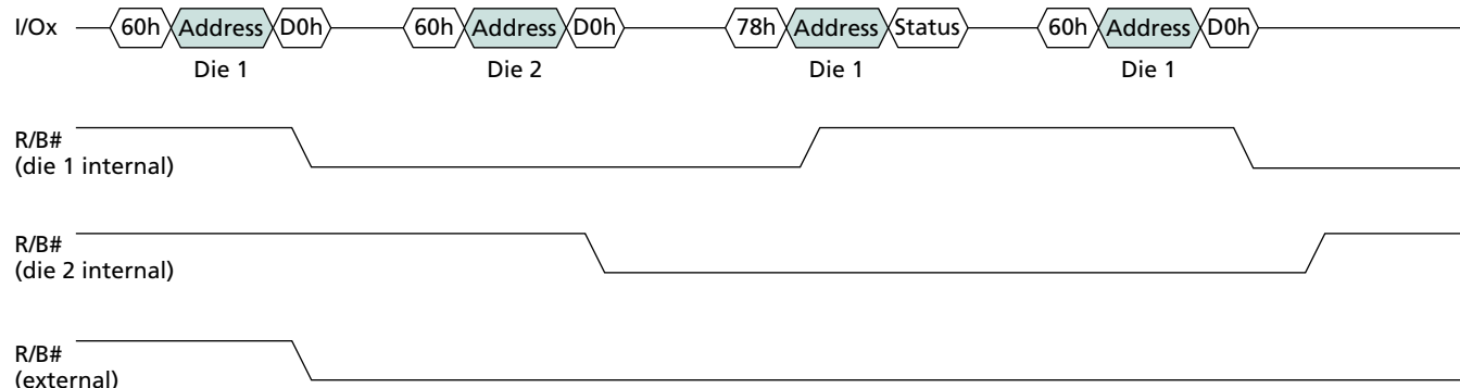
Figure 44: Interleaved BLOCK ERASE Operation with Status Register Monitoring
