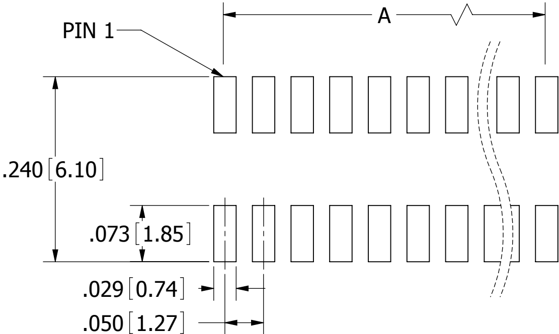
RECOMMENDED PCB SMD LAYOUT
