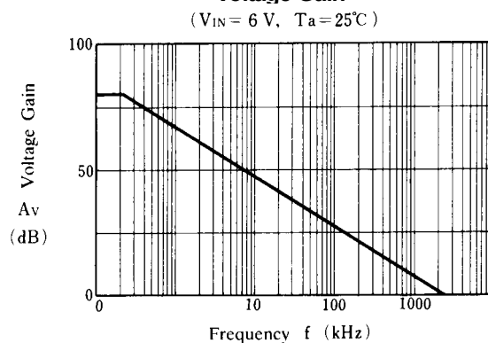
Voltage Gain
