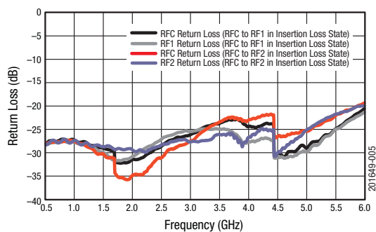
Figure 5. Return Loss vs Frequency (Insertion Loss State)
