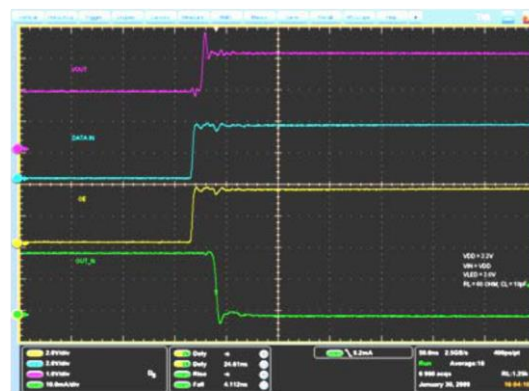
Figure 17: Turn OFF output current characteristics (2)
