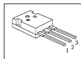
TO247-3-1
