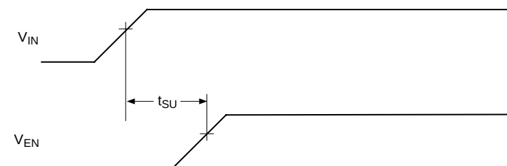
Figure 1c. Input-to-Enable Setup Timing
