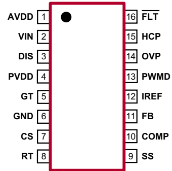
16-Lead SOIC
