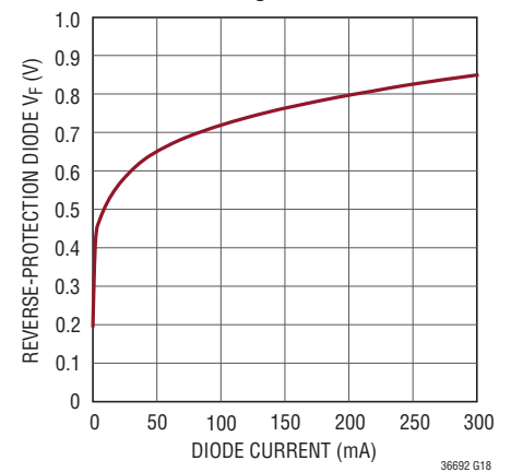
Reverse-Protection Diode Forward Voltage
