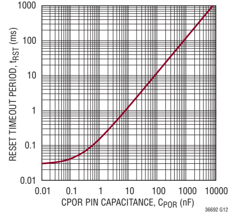
Reset Timeout Period
