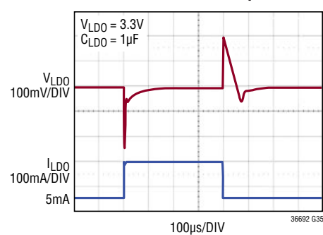
LDO Load Transient Response
