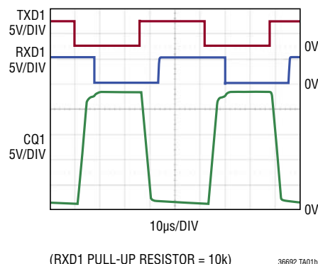
Operating Waveforms
