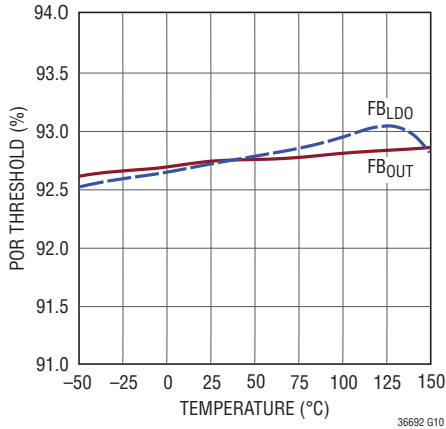
Power-On Reset Threshold
