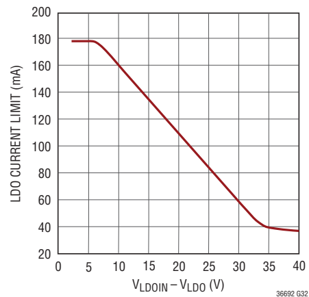
LDO Current Limit Foldback
