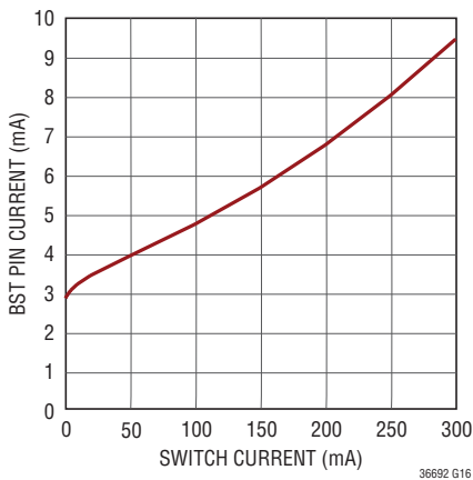
BST Pin Current
