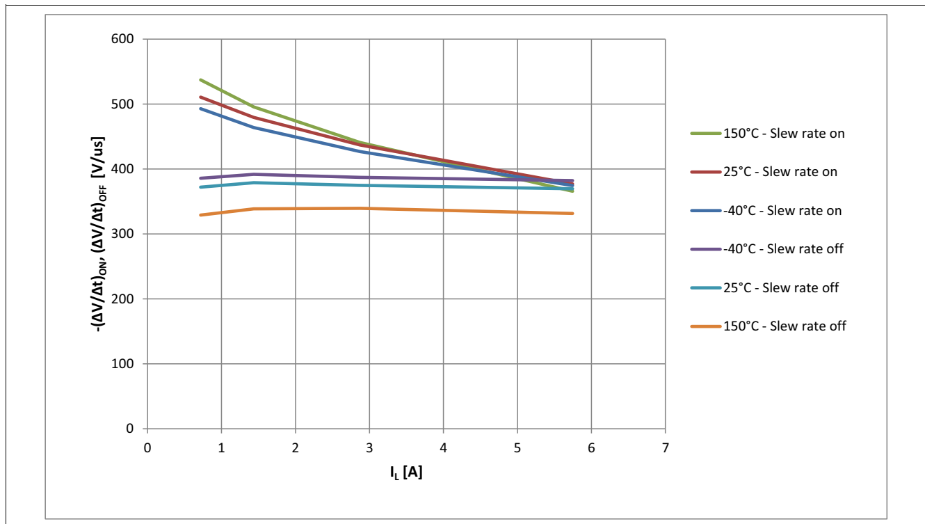
Figure 34 Typical -(\Delta V/\Delta t)_{ON} , (\Delta V/\Delta t)_{OFF} vs I_L @ V_{IN} = 5 V, T_J = -40 \dots 150^\circ\text{C}
