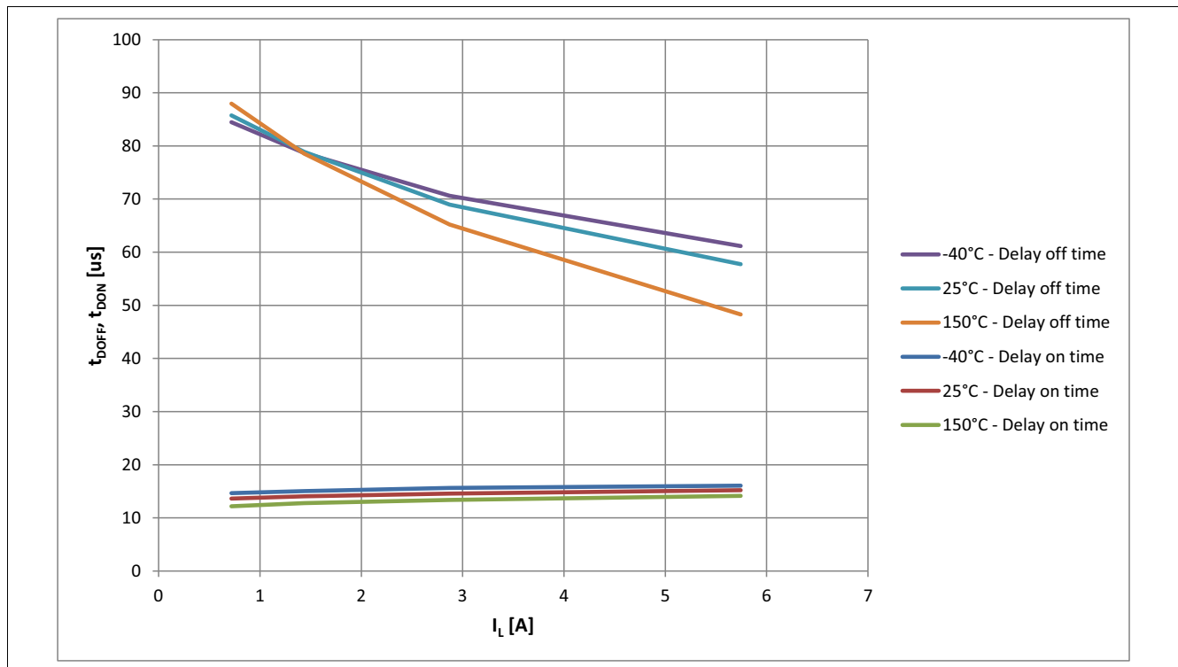
Figure 33 Typical t_{DON} , t_{DOFF} vs I_L @ V_{IN} = 5 V, T_J = -40 \dots 150^\circ\text{C}
