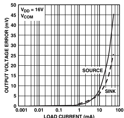
TPC 18. Output Voltage Error vs. Load Current
