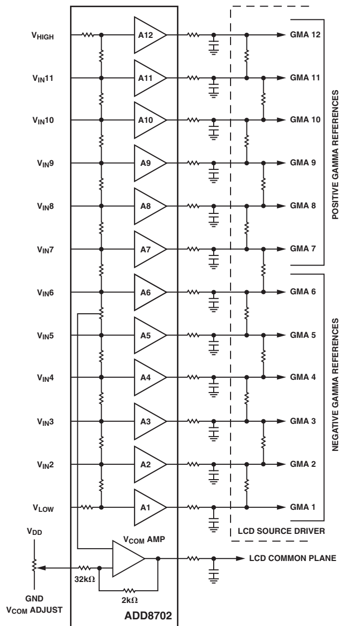
Figure 4. Application Circuit
