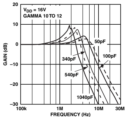
TPC 7. Frequency Response vs. Capacitive Loading
