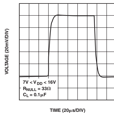
TPC 12. Small Signal Transient Response
