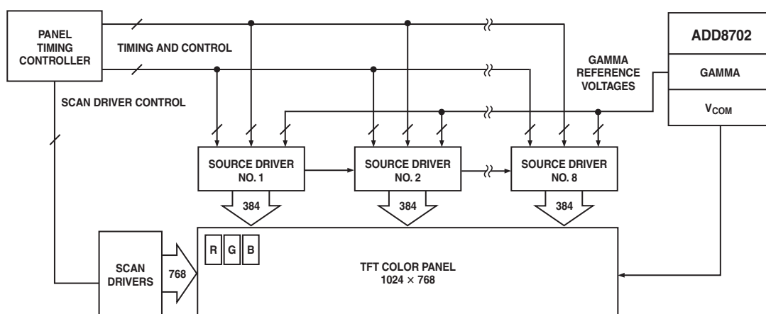
Figure 1. Typical SVGA TFT LCD Application
