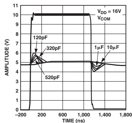
TPC 15. Transient Load Response vs. Capacitive Load
