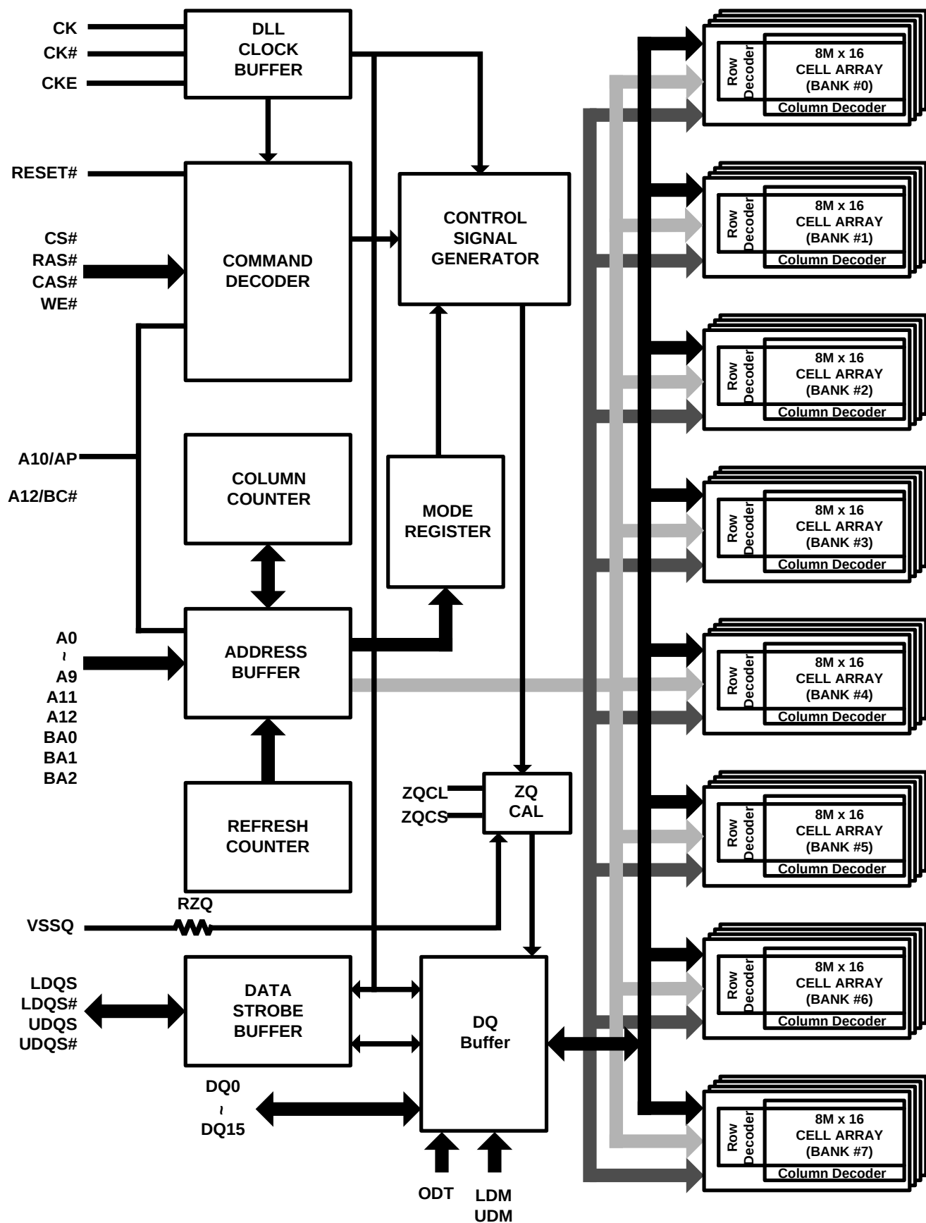
Figure 2. Block Diagram
