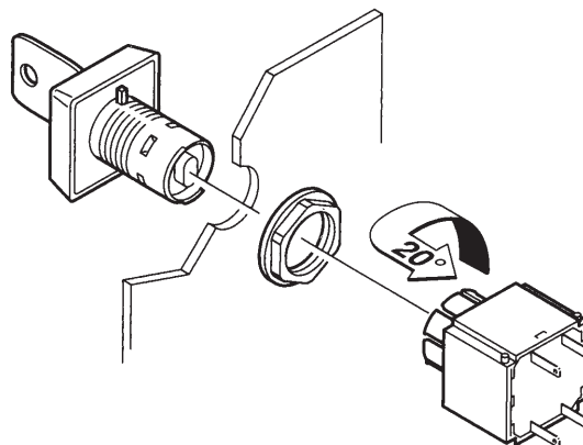
Assembly/Disassembly
