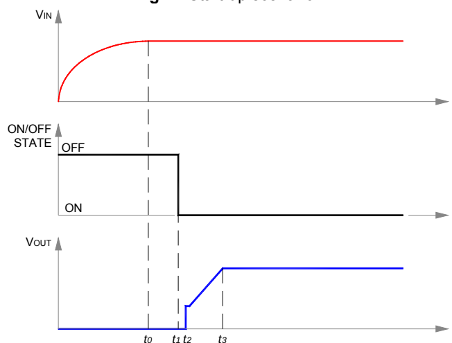
Fig. 8: Start-up scenario #2.
