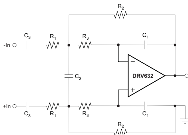
Figure 6. Differential Input, Second-Order Active Low-Pass Filter
