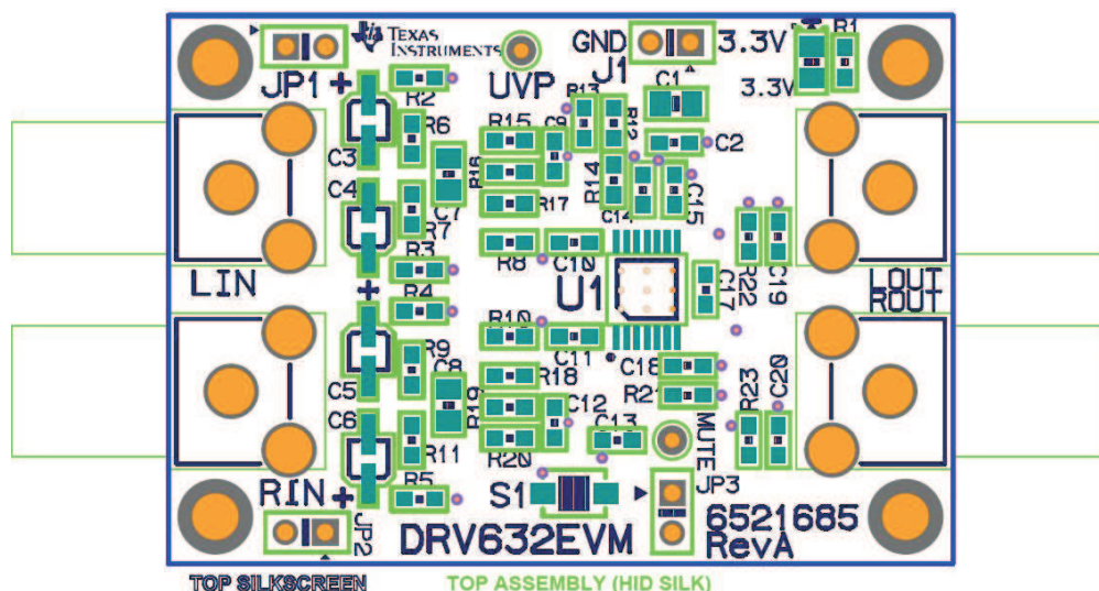
Figure 8. DRV632EVM PCB Component Placement
