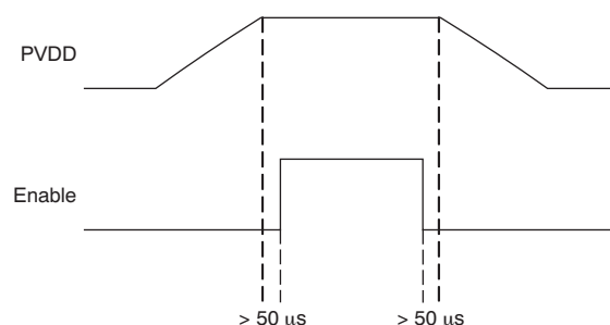
Figure 4. Power-Up/-Down Sequence
