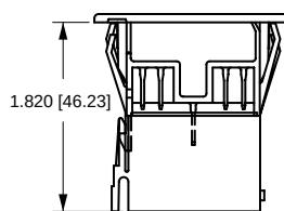
VH1 HOLE PLUG (No wing serrations) (With VC1 connector attached)
