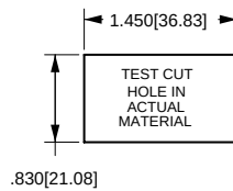
PLUG MOUNTING HOLE
