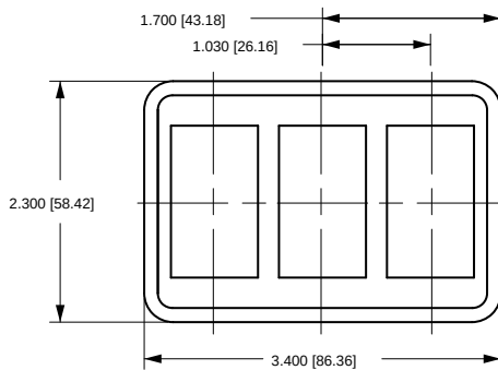
VM3 MOUNTING PANEL
