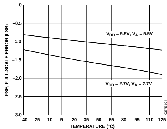
Figure 7. Full-Scale Error vs. Temperature
