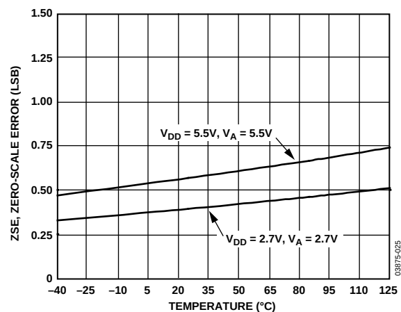
Figure 8. Zero-Scale Error vs. Temperature
