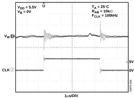
Figure 18. Digital Feedthrough
