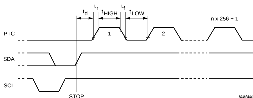
Fig.12 n bytes E/W cycle (n = 2 to 7).
