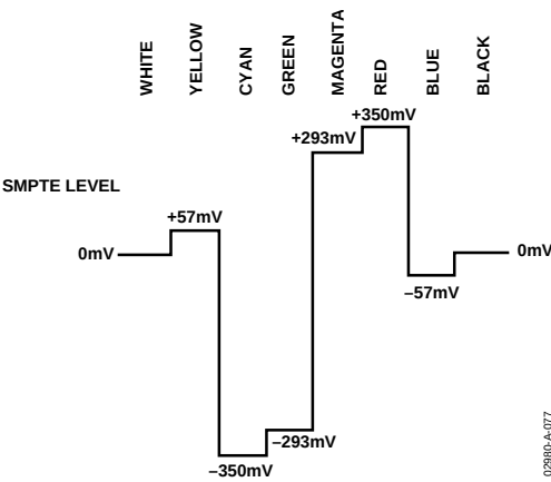
Figure 78. PAL 100% Color Bars, Pr Levels
