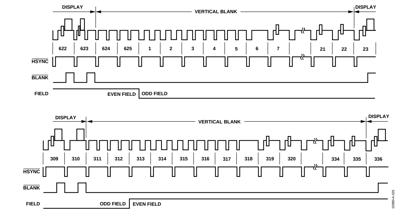
Figure 25. Timing Mode 1 (PAL)
