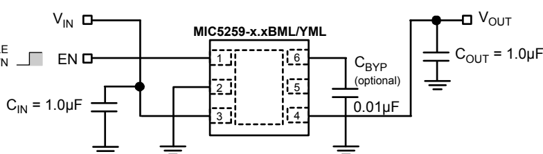
Ultra-Low Noise Regulator Application
