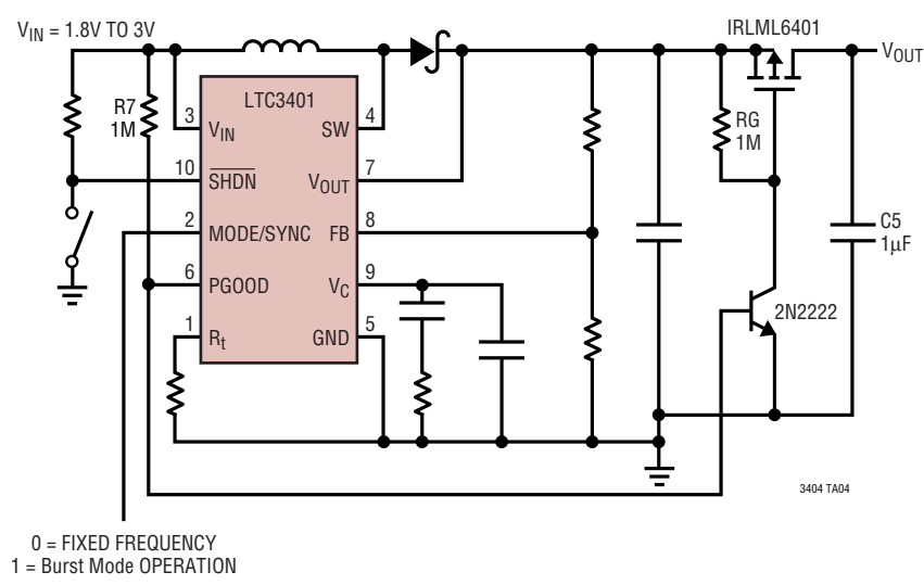
Dual Cell Output Disconnect Allowing Full Load Start-Up
