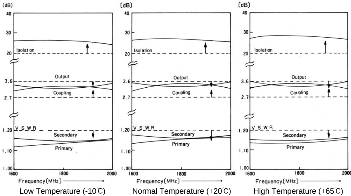
Temperature Test Data <HD-1800M3-CH>
