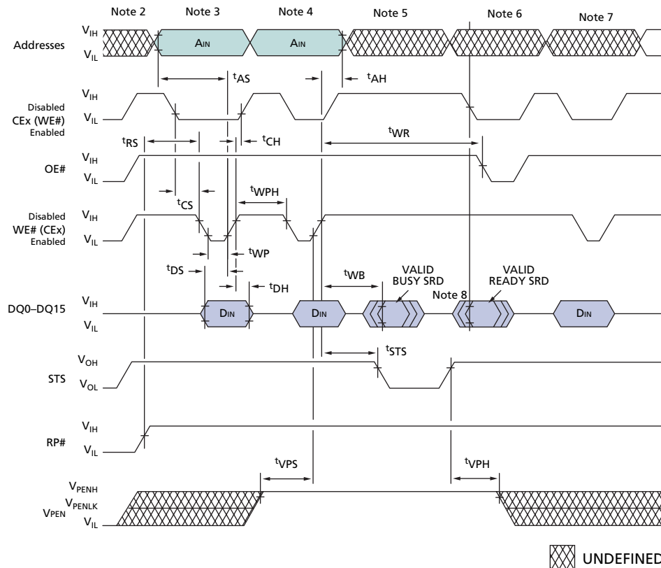
Figure 20: WRITE Operations
