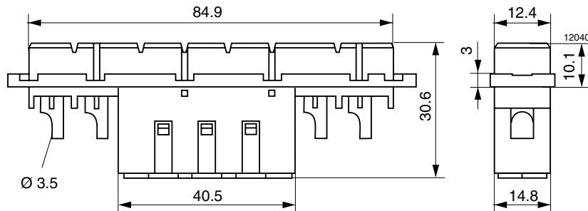
Fig. 12 STV-H15 S4-FLS/CO, screw terminals and four high current soldering terminals
