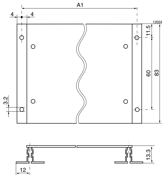
Fig. 4 "CMB" chassis mounting bracket dimensions Bracket: Aluminium, black finish
