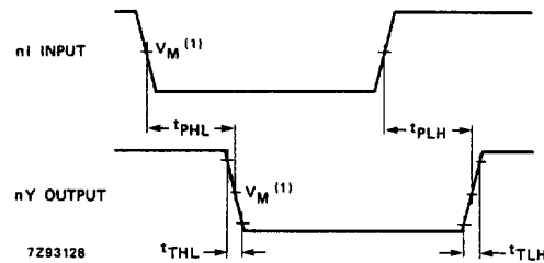
Fig.6 Waveforms showing the input ( 1I_n, 2I_n ) to output ( 1Y, 2Y ) propagation delays and the output transition times.
