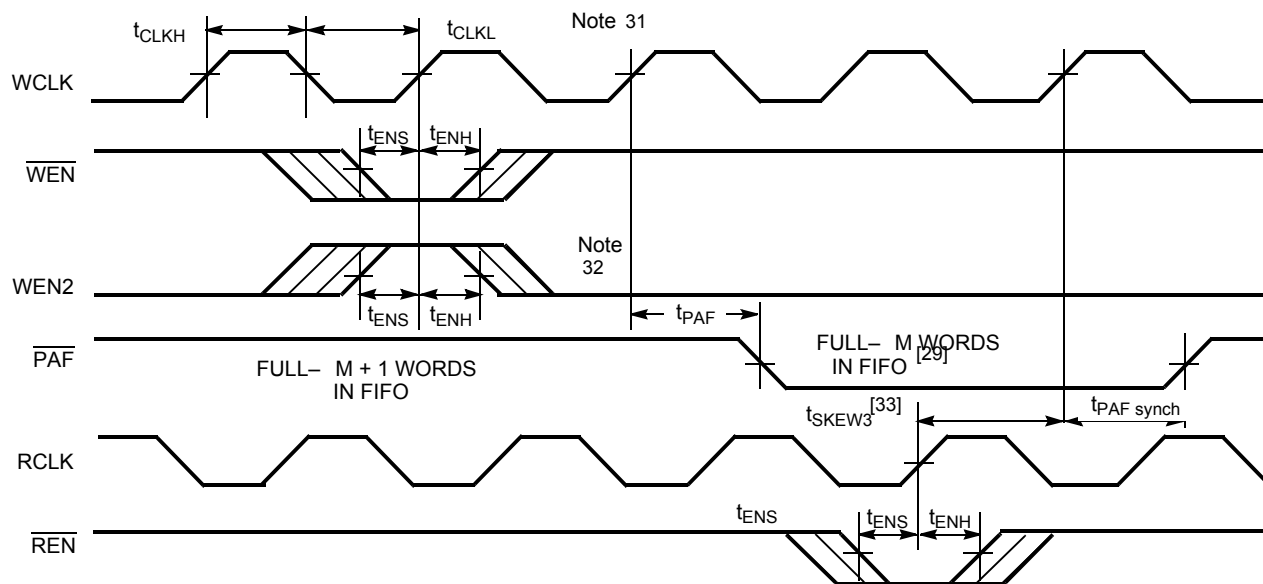
Figure 13. Programmable Almost Full Flag Timing (applies only in \overline{\text{SMODE}} ( \overline{\text{SMODE}} is LOW))
