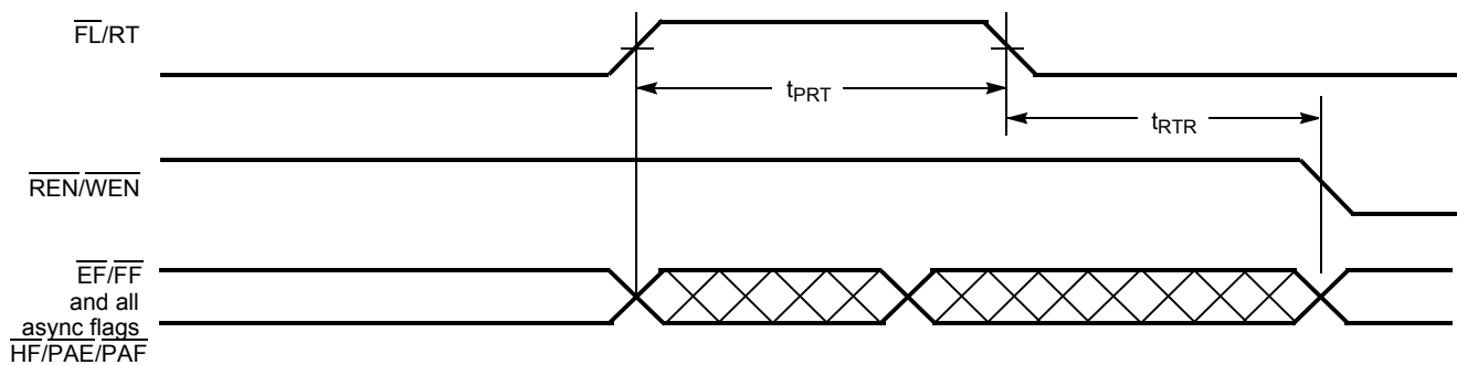
Figure 20. Retransmit Timing [36, 37, 38]
