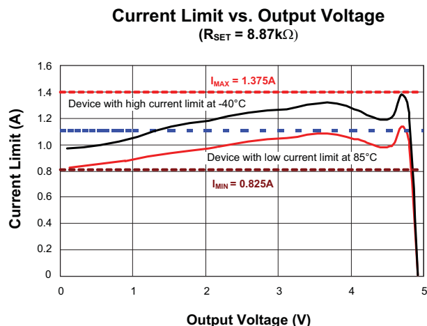
Figure 1: Current Limit Using 10.5k\Omega .
