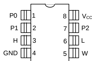
8-Pin SOIC (150-mil) See Mech. Drawings Section
