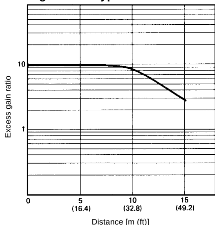
Through-Beam Type
