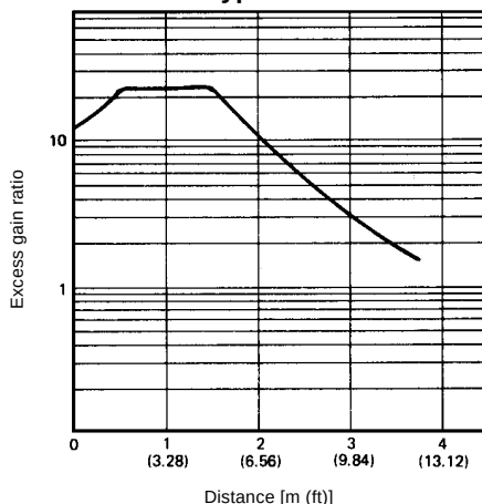
Retroreflective Type
