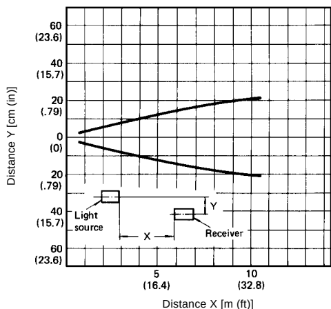
Through-Beam Type
