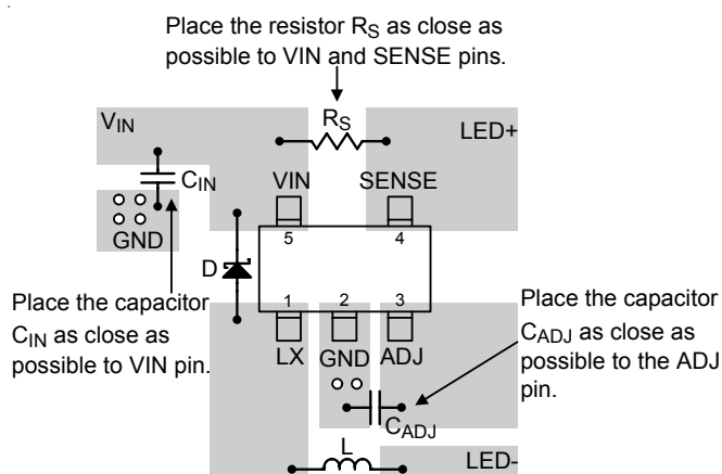
Figure 3. PCB Layout Guide
