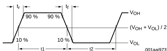
Fig 11. Definition of output and input transition times
