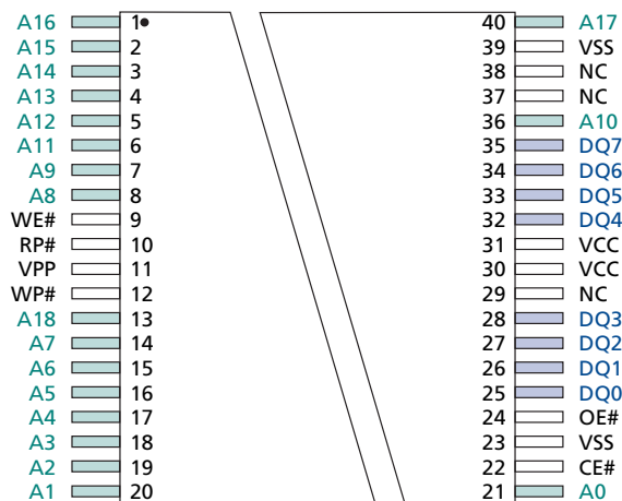
40-Pin TSOP Type I
