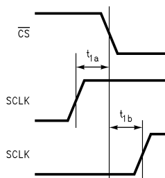
Figure 5. SCLK and \overline{CS} Timing Parameters
