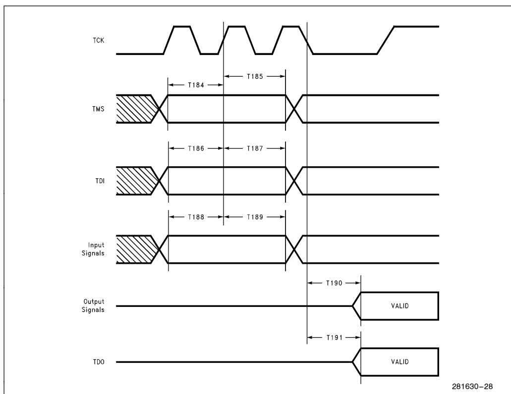
Figure 11-18. 82595TX JTAG Timing
