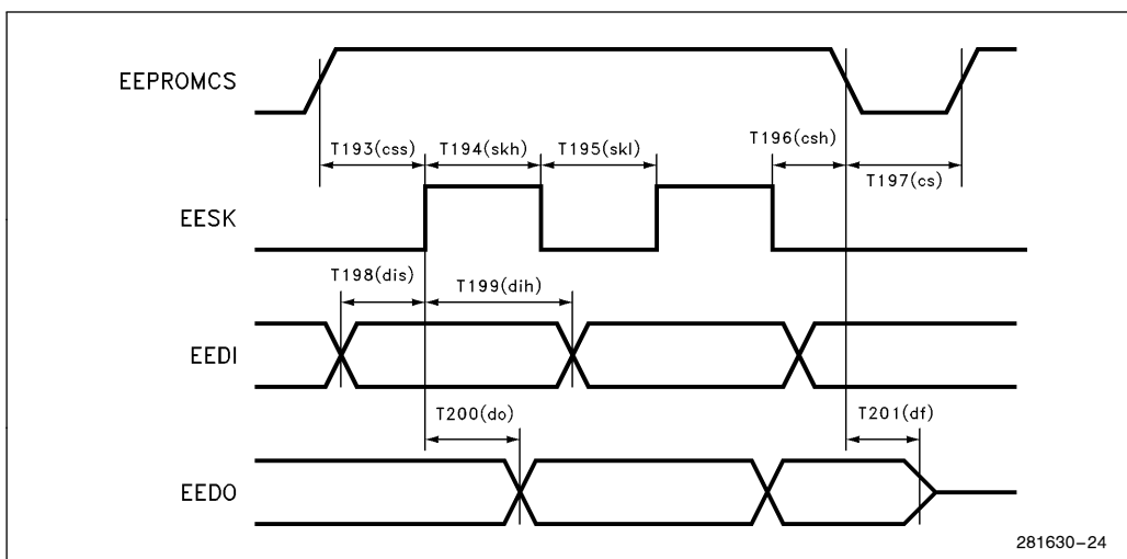
Figure 11-14. EEPROM Timings
