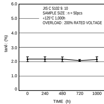
Fig.20 \tan\delta
