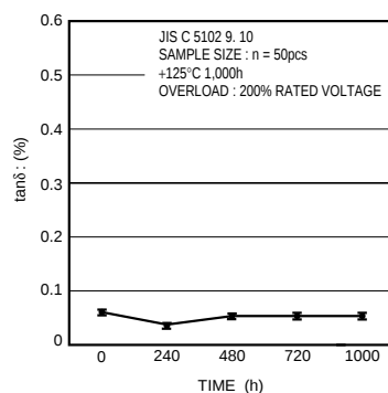
Fig.17 \tan\delta
