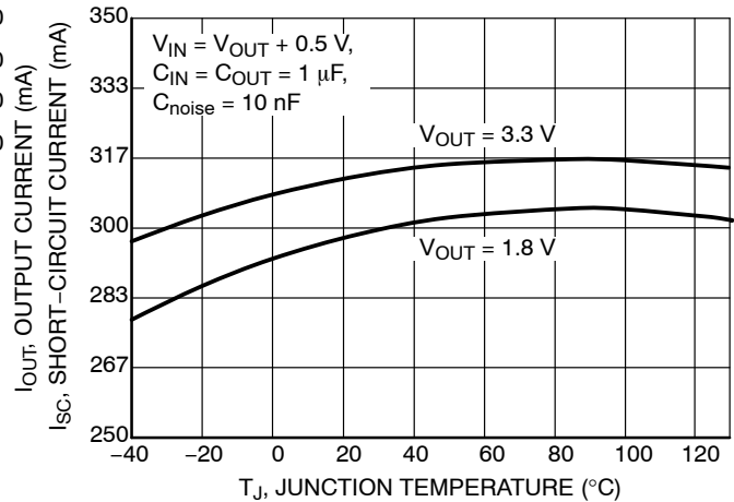
Figure 42. Short-Circuit Current vs. Junction Temperature, V_{OUT} = 1.8 V, 3.3 V
