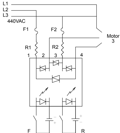
Foward / Reverse Motor Control Wire Diagram
